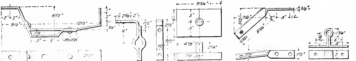
Figs. 775-6. Floating Lever Fulcrum (1). Figs. 777-8. Pipe Clamps (2). Figs. 779-80. Follower Plates (4). Figs. 781-2. Hose Hook Coupling Iron (2). Figs. 783-81. Shaft Collar (1).
